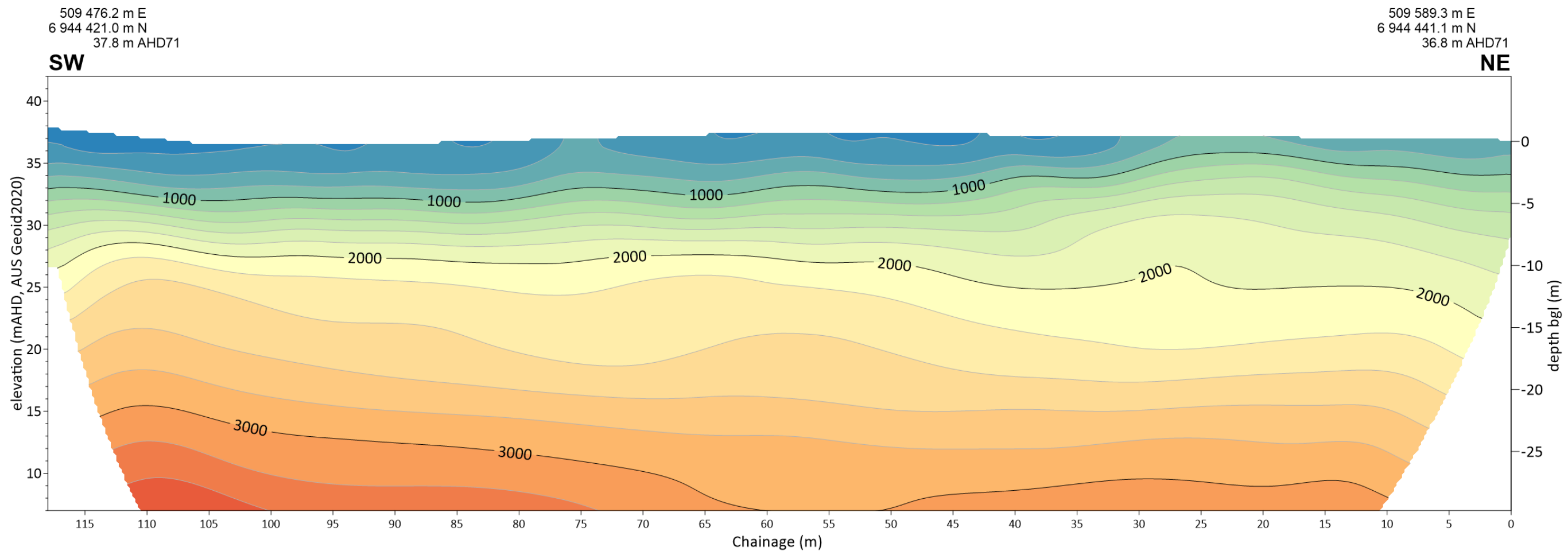
Seismic Line SR AU-GP 118
